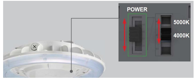
CCT Color and Lumen/Wattage Selectable Switches
